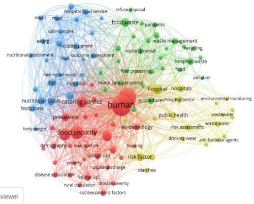
Figure 6. Network Visualization.
